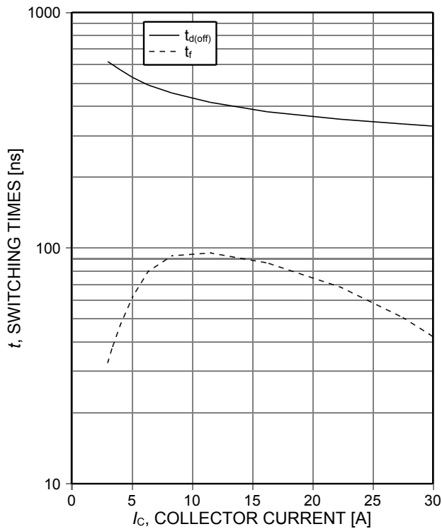
Figure 9. Typical switching times as a function of collector current (ind. load, T_J=175^{\circ}\text{C} , V_{CE}=600\text{V} , V_{GE}=0/15\text{V} , R_{G(on)}=14,6\Omega , R_{G(off)}=14,6\Omega , test circuit in Fig. E)
