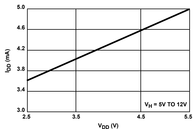
FIGURE 8. QUIESCENT I_{DD} vs V_{DD}
