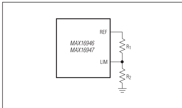
Figure 6. Current-Limit Threshold Selection
