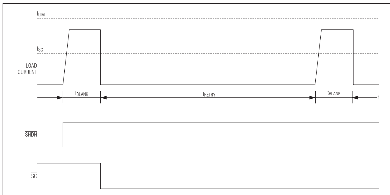
Figure 4. Turn-On into Heavy Load
