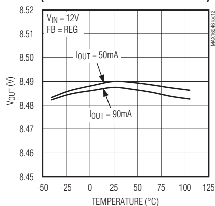
OUTPUT VOLTAGE vs. TEMPERATURE (MAX16946 8.5V LDO CONFIGURATION)
