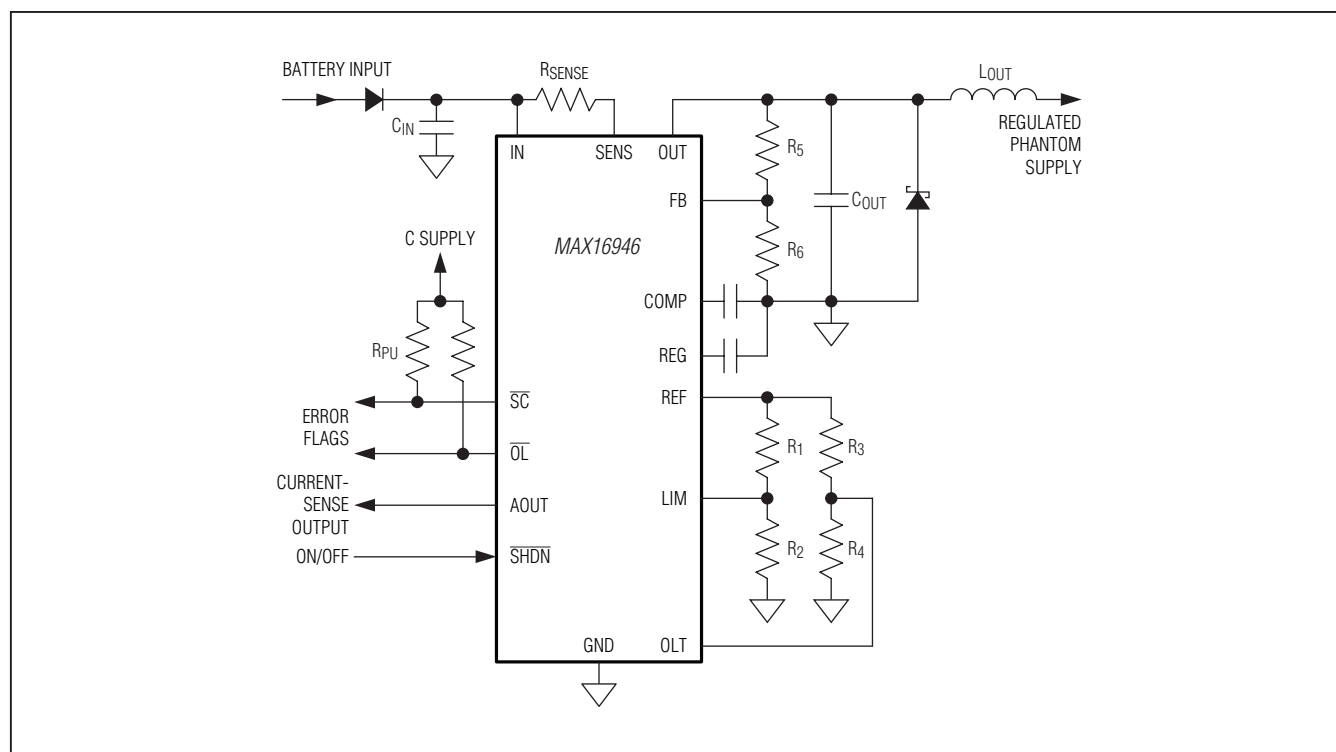
Figure 8. LDO with Adjustable Output Voltage (3.3V to 15V)
