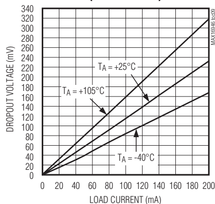
DROPOUT VOLTAGE vs. LOAD CURRENT (OUTPUT = 8.5V)
