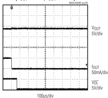
OPEN-LOAD FAULT ( V_{OUT} = 8.5V , I_{OUT} = 50mA )
