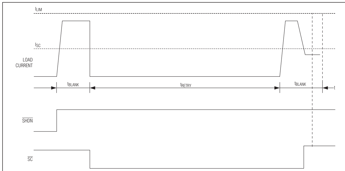
Figure 3. Turn-On into Temporary Heavy Load
