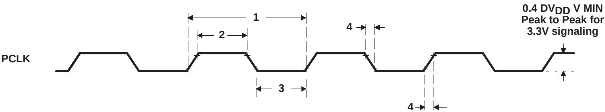
Figure 47. PCLK Timing
