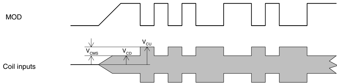
Figure 4-1. Modulation
