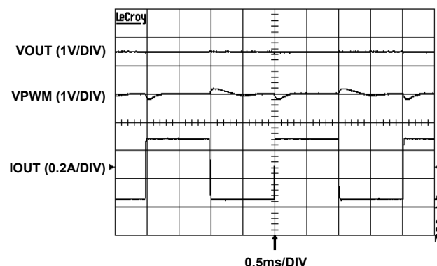
FIGURE 11. DYNAMIC RESPONSE VOUT = 14.0V
