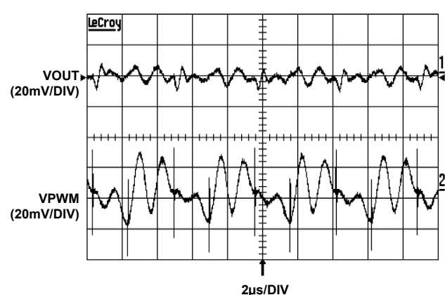
FIGURE 9. RIPPLE VOUT = 18.0V
