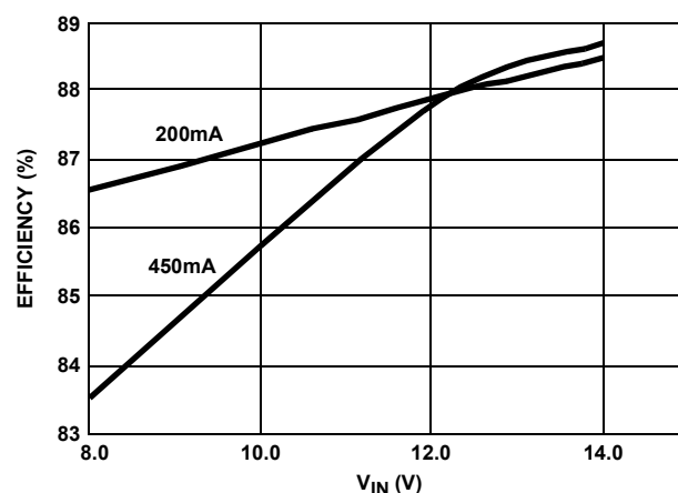
FIGURE 5. EFFICIENCY vs VIN
