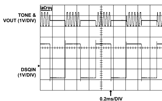
FIGURE 7. 22kHz TONE MODULATED BY DSQIN
