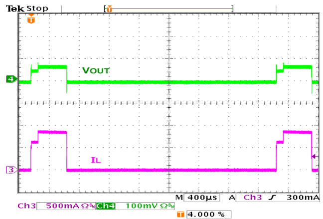
Figure 35. Short-Circuit Response
