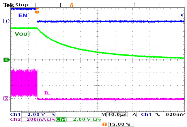
Figure 33. Shutdown, 33 \Omega Load
