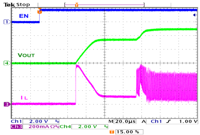
Figure 31. Startup, 33 \Omega Load
