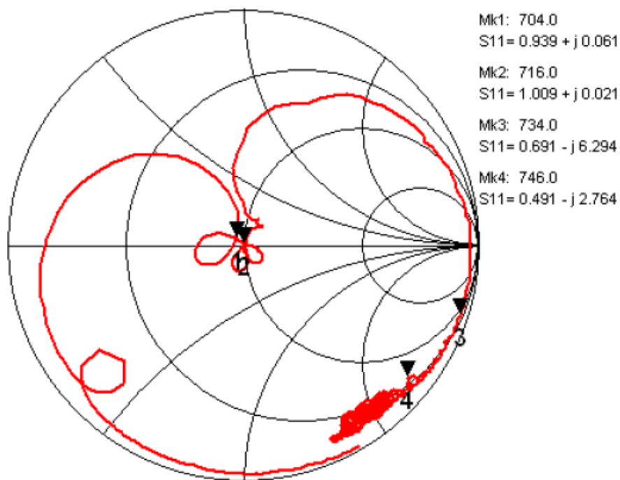
Fig.5 Impedance (INPUT)
