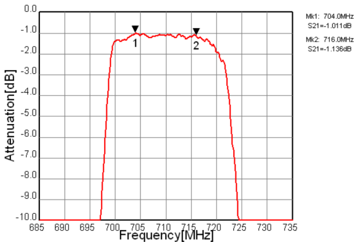
Fig.2 In-band Characteristic
