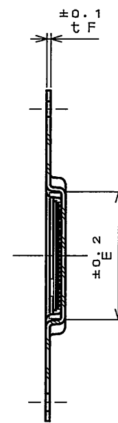
SECT. C-C (SCALE 2:1)
