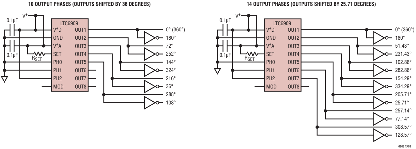
Using Additional Standard Logic Inverters to Achieve 10- and 14-Phase Outputs (Inverters Are 74HC04 or Equivalent)
