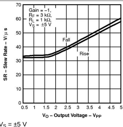
Figure 31. Slew Rate
