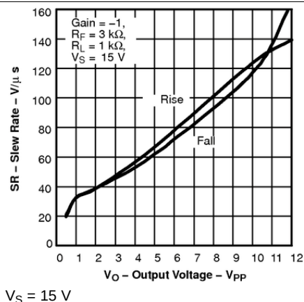
Figure 32. Slew Rate
