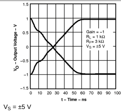
Figure 37. Settling Time
