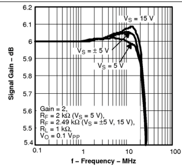
Figure 14. Frequency Response
