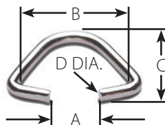
OPEN TRIANGLE RINGS (NON-TEMPERED STEEL)
