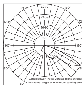
ITL Test Report #: 72722 BXSPA*G2A-U Initial Delivered Lumens: 3,427
