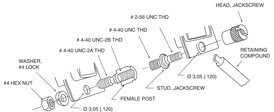
Jackscrew Assembly
