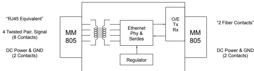
Block Diagram
