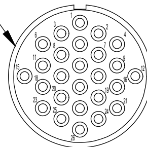
J2 Mighty Mouse Connector Series 805 Size 11
