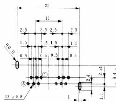
TM2RE-1212 (50)
