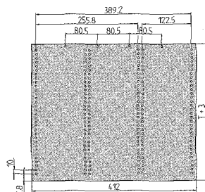
Cover plate for board mounting
