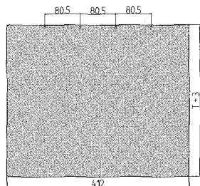
Plain cover plate
