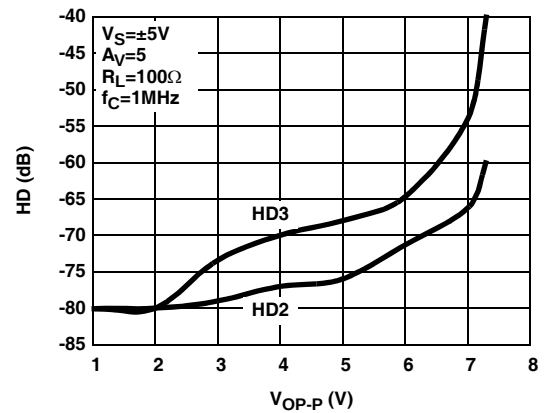
FIGURE 20. DIFFERENTIAL HARMONIC DISTORTION vs OUTPUT AMPLITUDE (FULL POWER)
