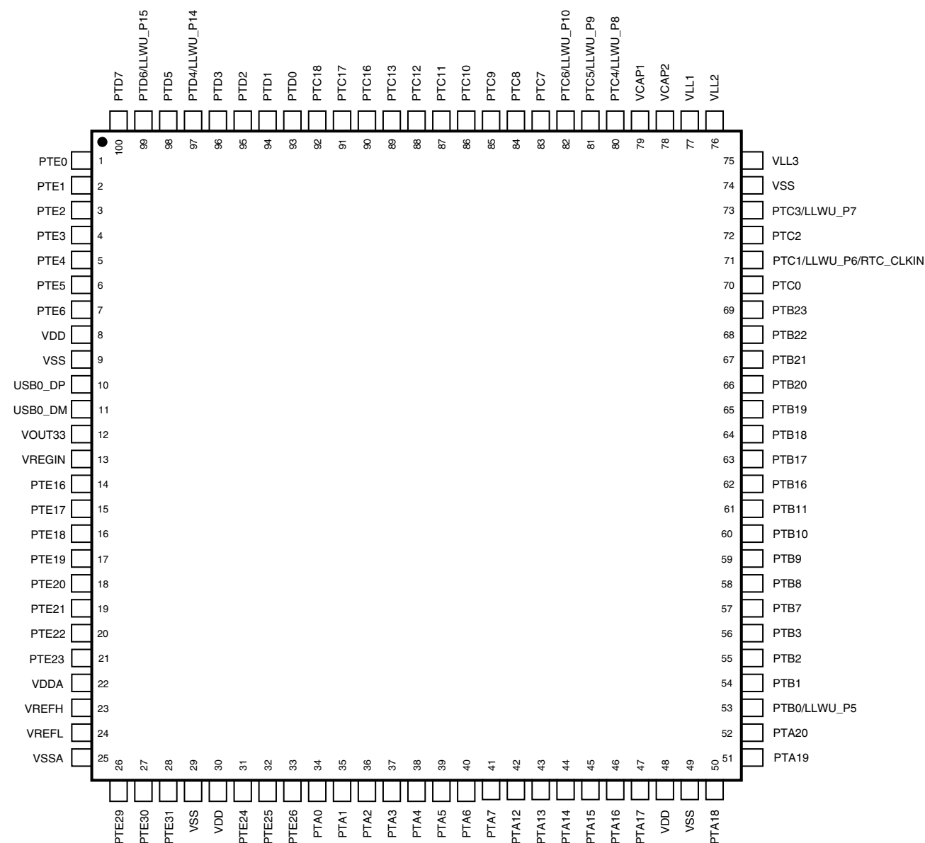
Figure 23. KL46 100-pin LQFP pinout diagram
