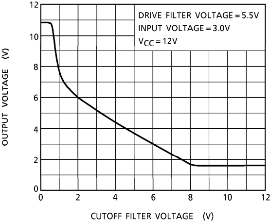
Fig.1 Cutoff control characteristics
