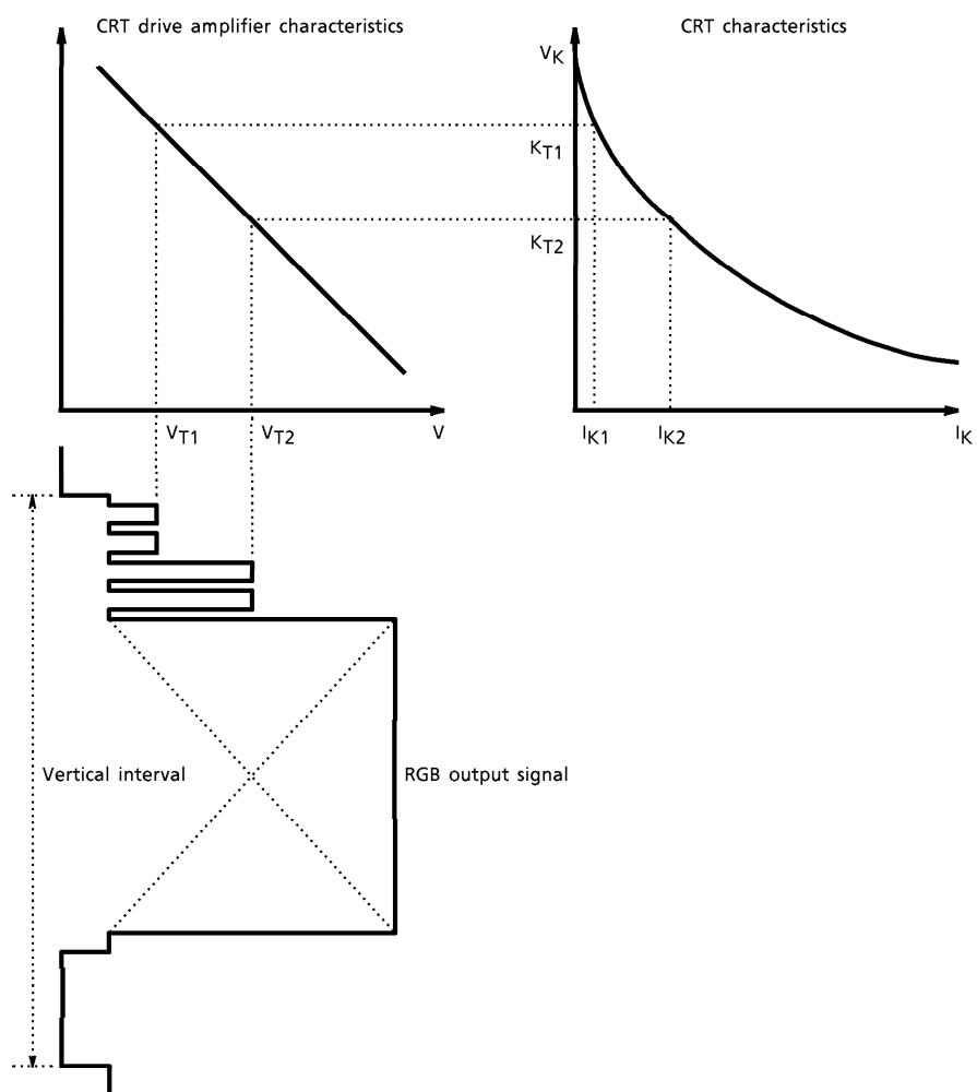
Fig.4 Basic structure of CRT drive circuit
