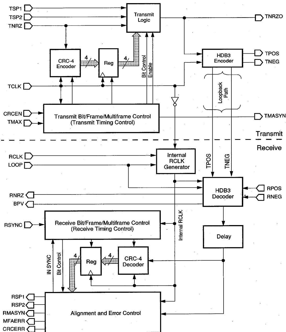
Figure 4. Bt8075 Functional Block Diagram
