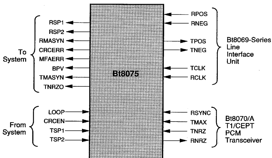
Figure 2. Bt8075 Interface Signals
