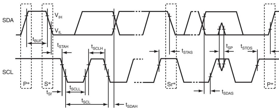
Figure 21.3 Input Timing
