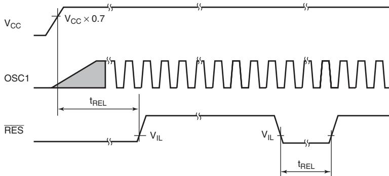
Figure 21.2 \overline{\text{RES}} Low Width Timing
