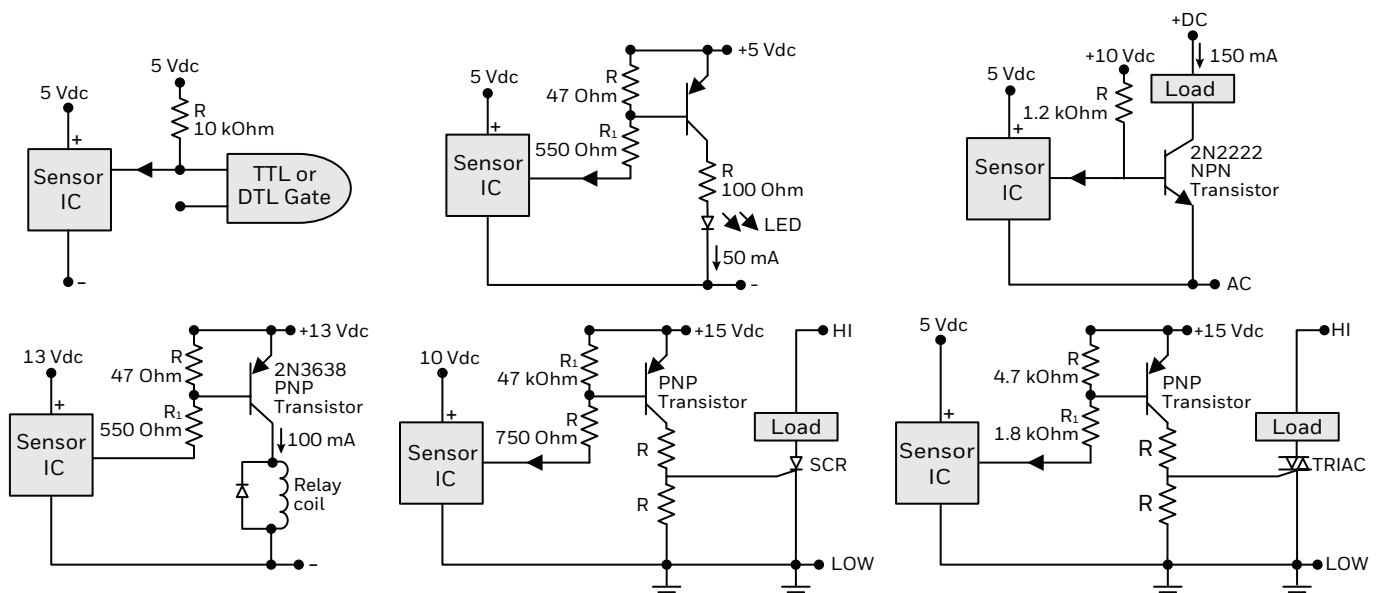
Figure 3. Circuit Diagrams
