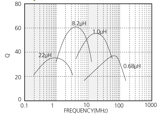
■ Q CHARACTERISTICS
