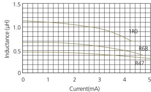
DC BIAS CHARACTERISTIC
