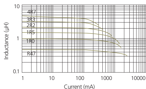
DC BIAS CHARACTERISTIC(Typ.)
