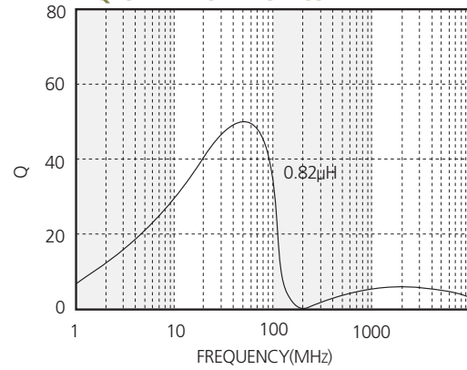
■ Q CHARACTERISTICS
