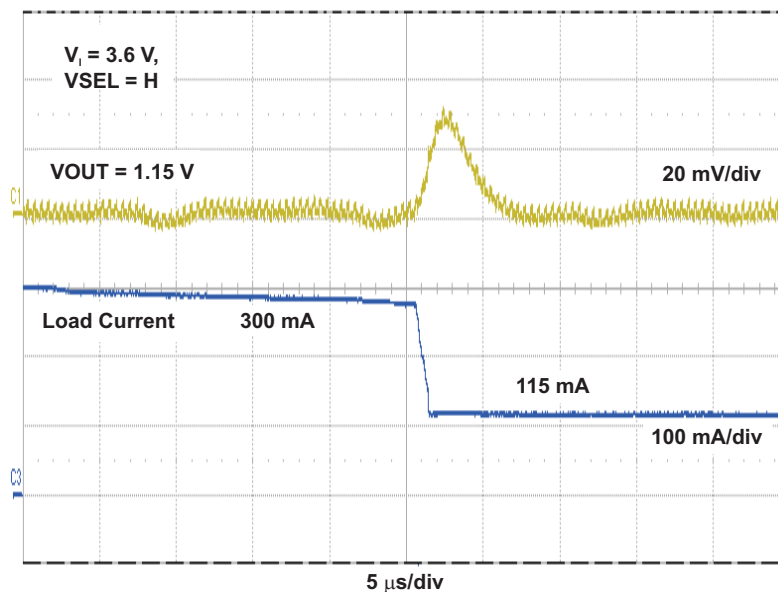
Figure 3. Load Transient, 300 mA to 115 mA step, V_I = 3.6\text{ V} , V_{OUT} = 1.15\text{ V}
