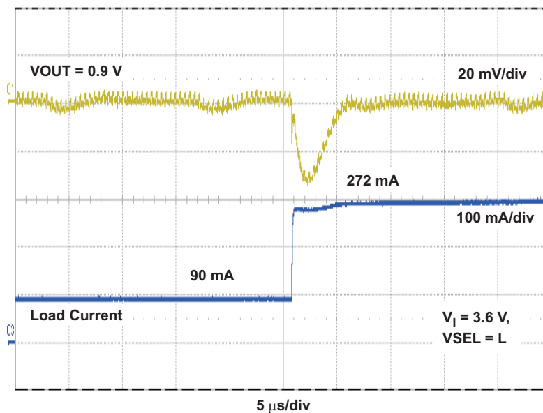
Figure 5. Load Transient, 90 mA to 272 mA step, V_I = 3.6 \text{ V} , VOUT = 0.9 \text{ V}
