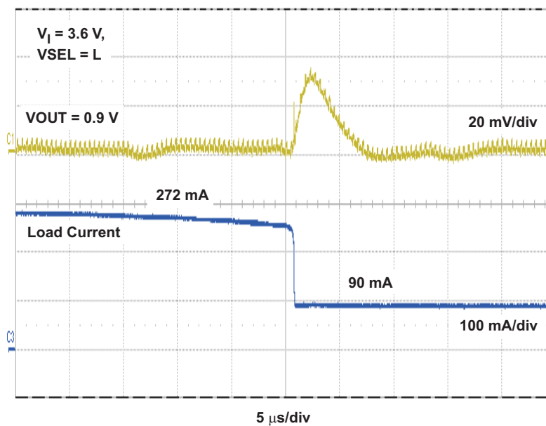
Figure 6. Load Transient, 272 mA to 90 mA step, V_I = 3.6 \text{ V} , VOUT = 0.9 \text{ V}
