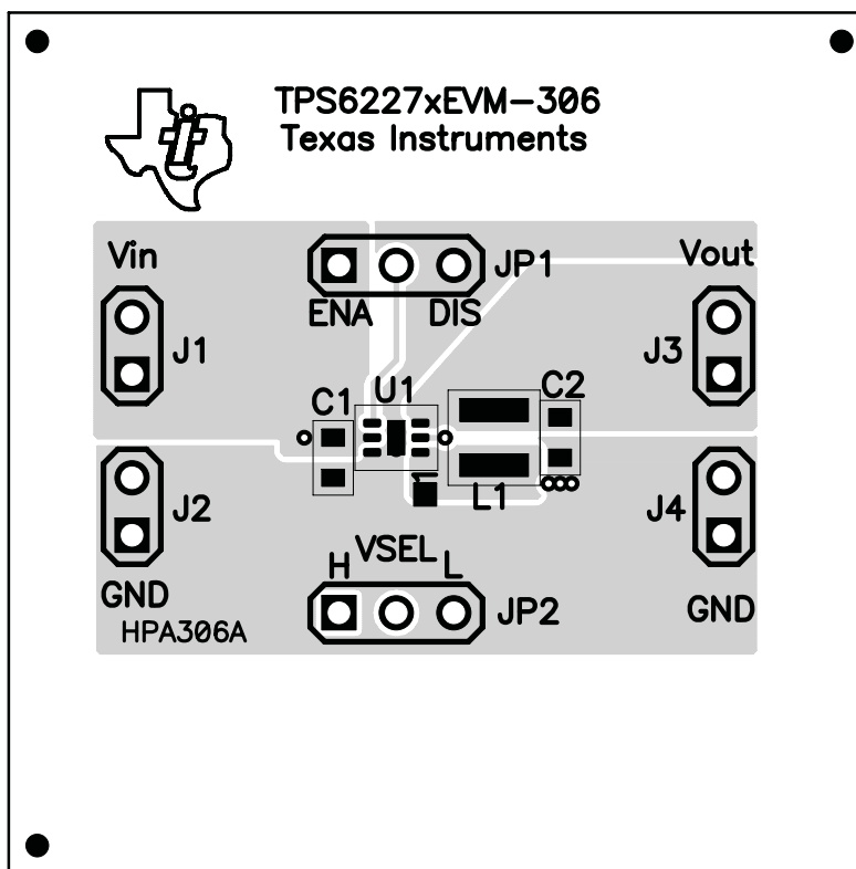
Figure 8. Assembly Layer
