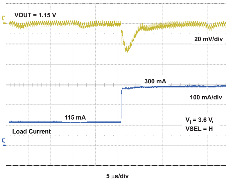
Figure 2. Load Transient, 115 mA to 300 mA step, V_I = 3.6 V, V_{OUT} = 1.15 V
