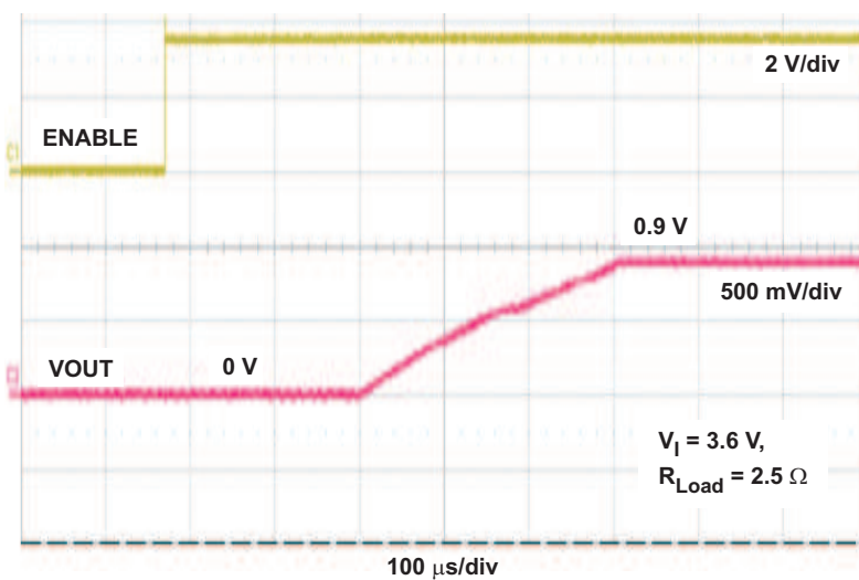
Figure 4. Start up from Enable, V_I = 3.6\text{ V} , V_{OUT} = 0.9\text{ V} , R_{Load} = 2.5\ \Omega
