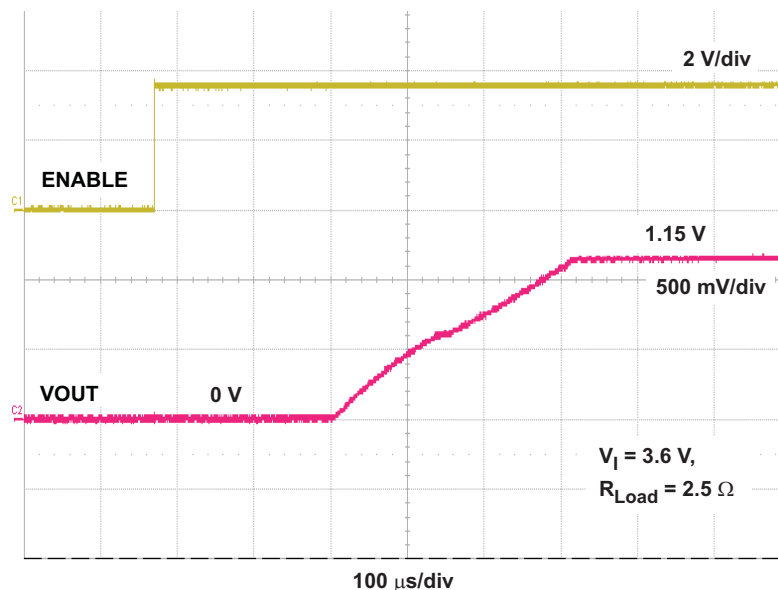
Figure 1. Start up from Enable, V_I = 3.6 V, V_{OUT} = 1.15 V, R_{Load} = 2.5 \Omega
