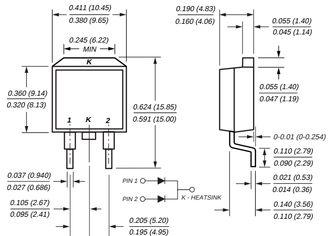
TO-263AB (MBRB10H90CT, MBRB10H100CT)
