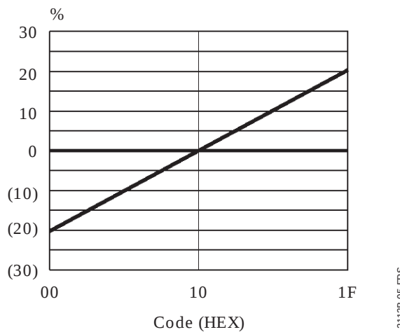
Figure 3 : Brightness Control Curve
