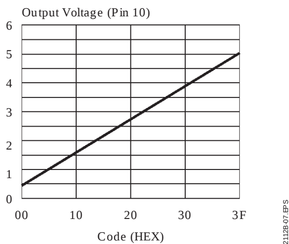
Figure 5 : Volume Control Curve
