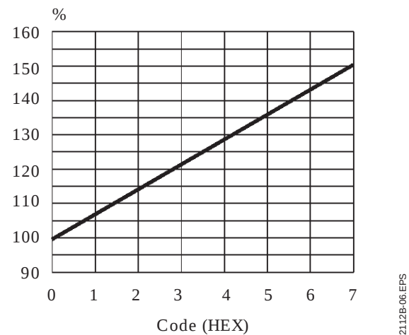
Figure 4 : Peaking Control (2T overshoot)
