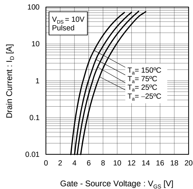
Fig.8 Typical Transfer Characteristics (I)
