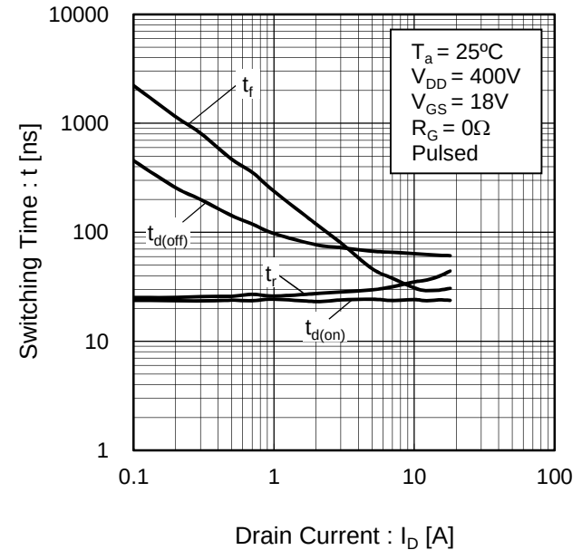
Fig.17 Switching Characteristics
