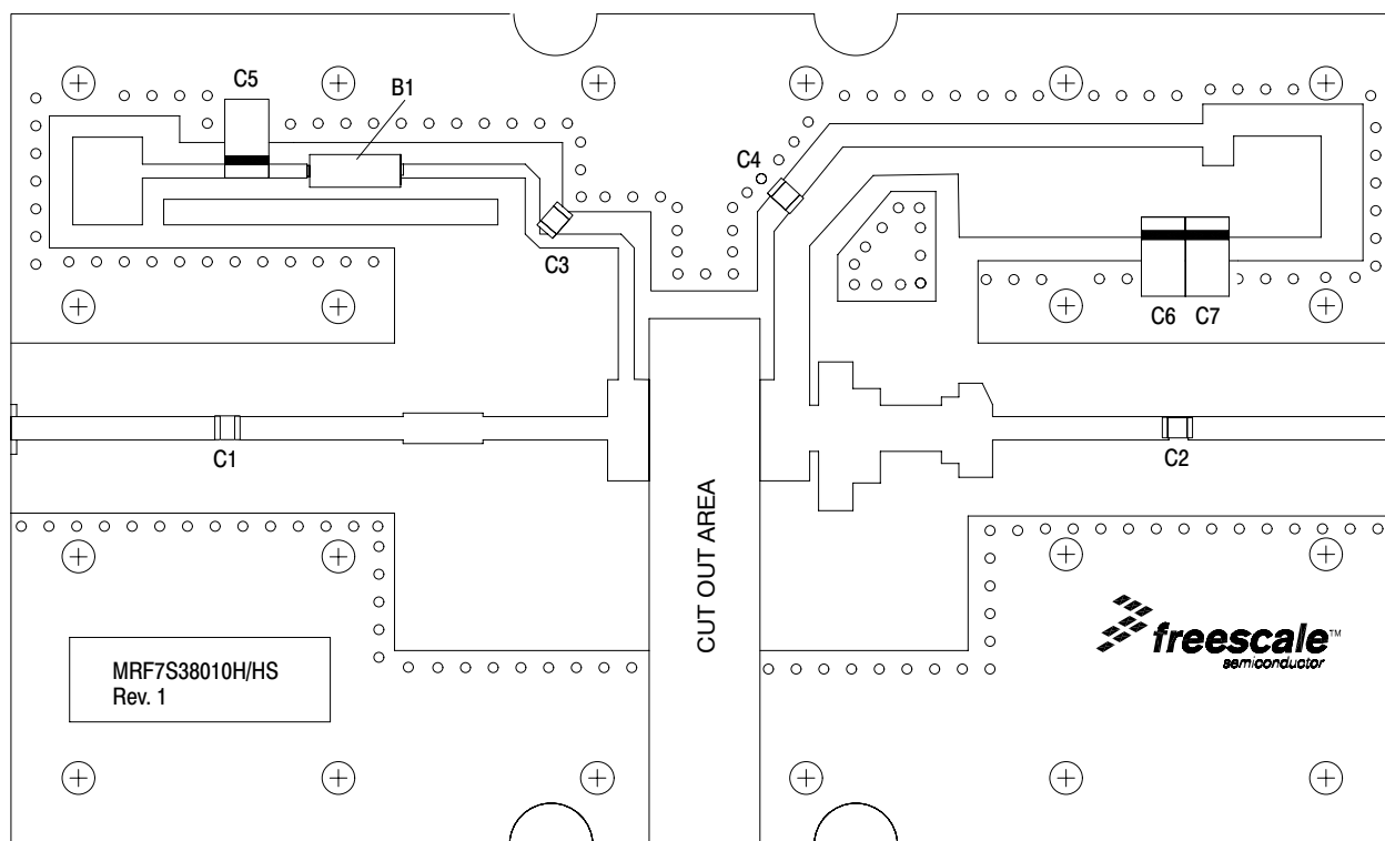
Figure 2. MRF7S38010HR3(HSR3) Test Circuit Component Layout
