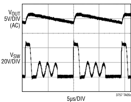
Switching Waveforms
