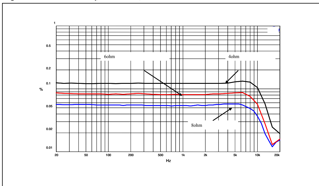
Figure 11. THD vs. Freq, V_{CC} = 18\text{ V} , P_o = 1\text{ W}
