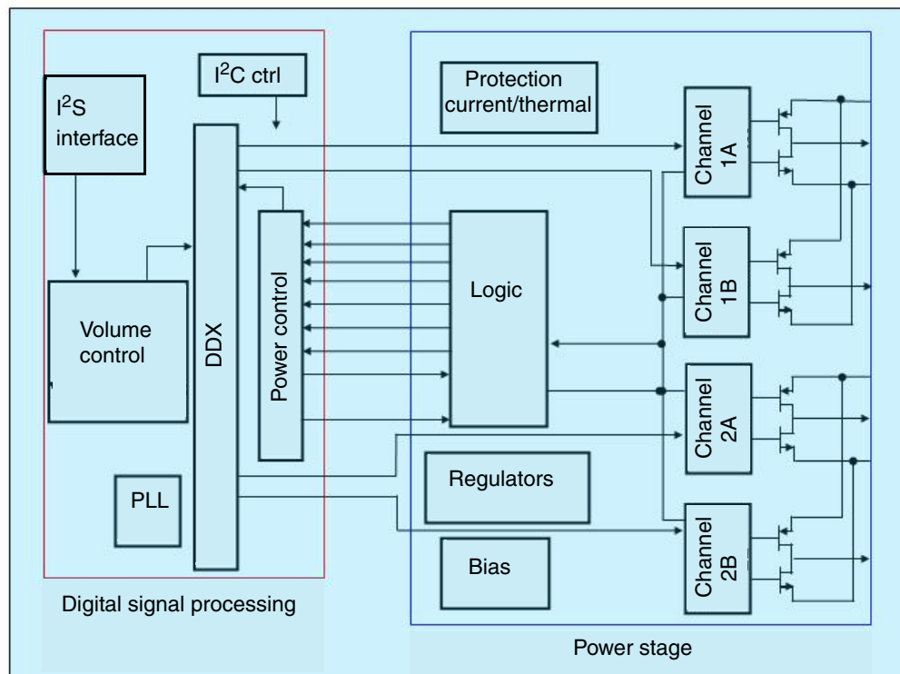
Figure 1. Block diagram
