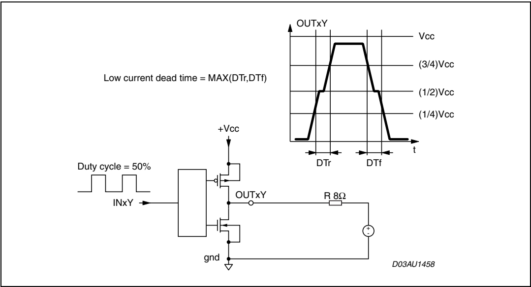
Figure 3. Test circuit
