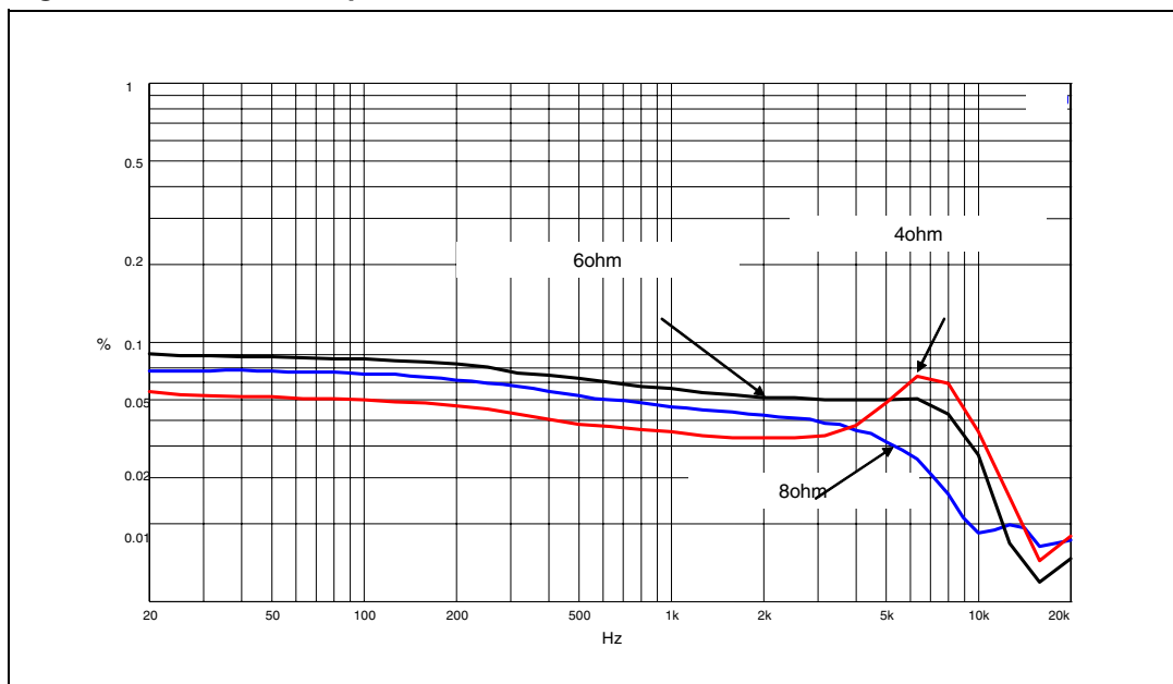
Figure 8. THD vs. Freq, V_{CC} = 12\text{ V} , P_o = 1\text{ W}
