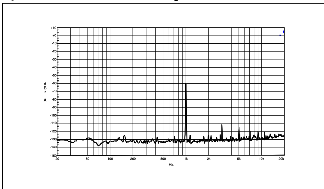
Figure 7. FFT -60 dBfs 1 kHz, V_{CC} = 12\text{ V} , R_L = 8\ \Omega
