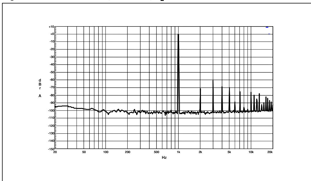
Figure 9. FFT 0 dBfs 1 kHz, V_{cc} = 18\text{ V} , R_L = 8\ \Omega
