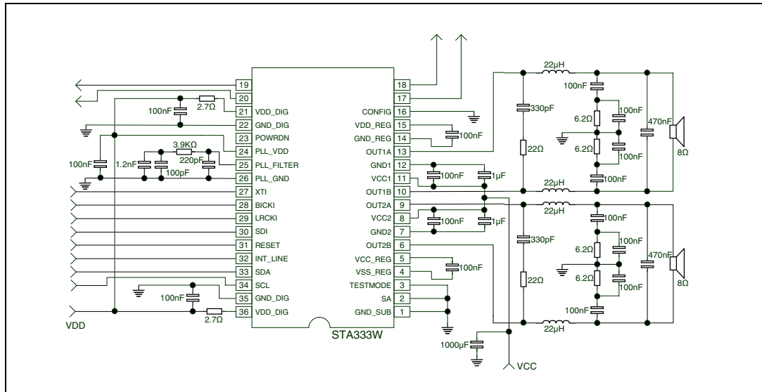
Figure 14. Application diagram
