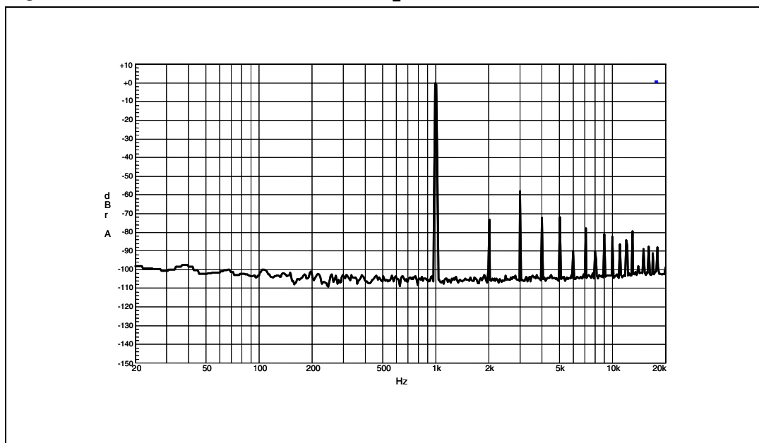
Figure 6. FFT 0 dBfs 1 kHz, V_{cc} = 12\text{ V} , R_L = 8\ \Omega
