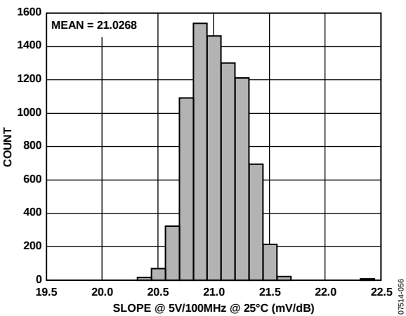
Figure 23. Slope Distribution, 100 MHz
