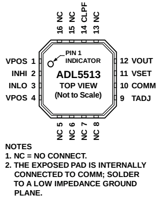
Figure 2. Pin Configuration
