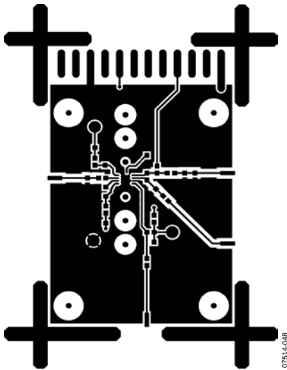
Figure 48. Component Side Layout
