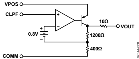
Figure 28. Output Interface
