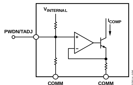
Figure 35. TADJ Interface
