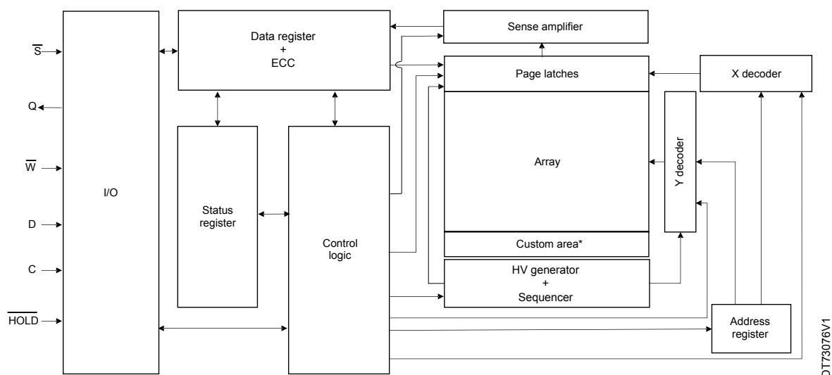
Figure 3. Block diagram
