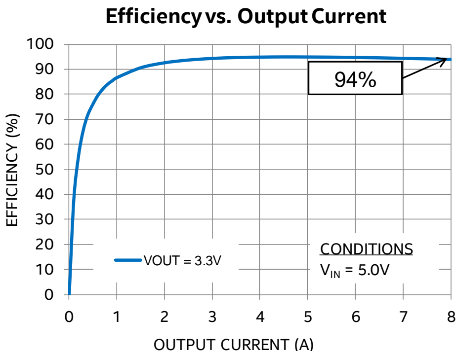
Figure 8: Efficiency vs. Output Current
