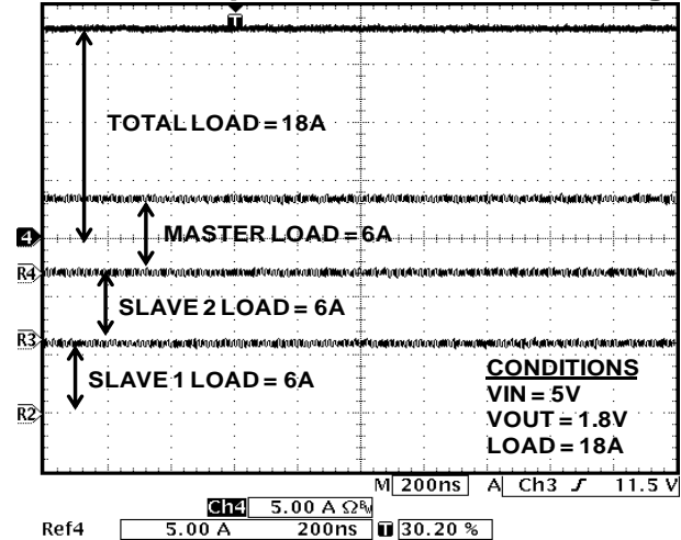
Parallel Operation Current Sharing
