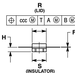
CASE 360B-05 ISSUE F NI-360 MRF9045LR1
