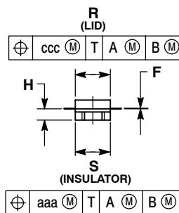
CASE 360C-05 ISSUE D NI-360S MRF9045LSR1
