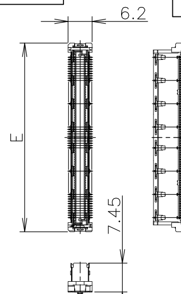
CONNECTOR DETAIL
