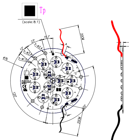
GLV91C76761/20 (with 200mm,20Awg wire)
