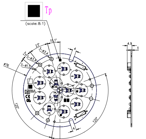
GLV91C76761/CN (with connector)
