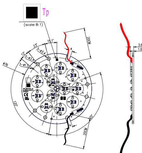
GLV92C76761/20 (with 200mm,20Awg wire)
