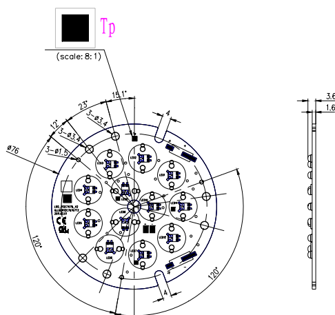
GLV92C76761/00 (with solder pads only)
