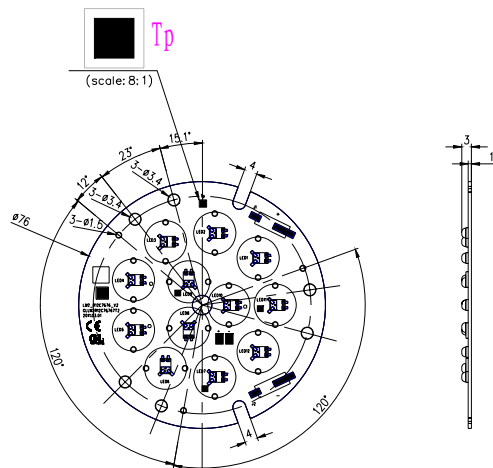
GLV91C76761/00 (with solder pads only)
