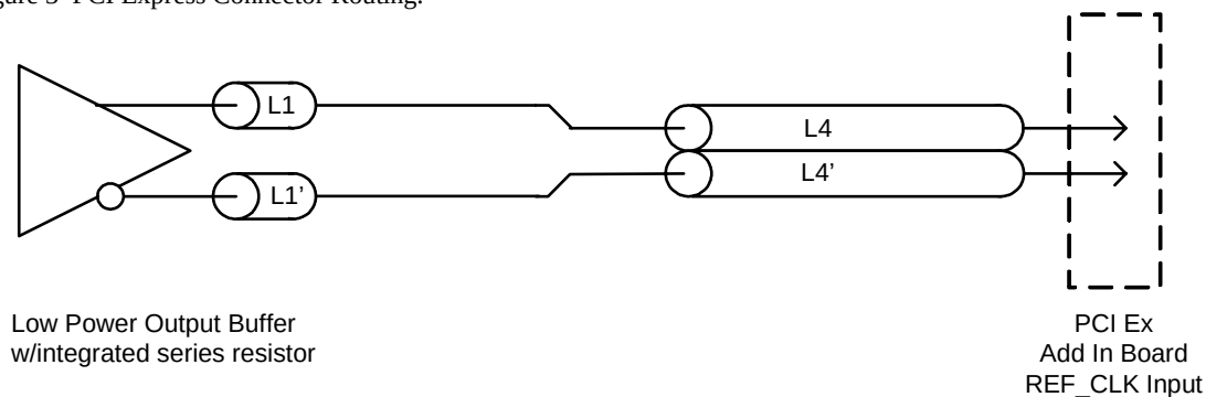
Figure 3 PCI Express Connector Routing.
