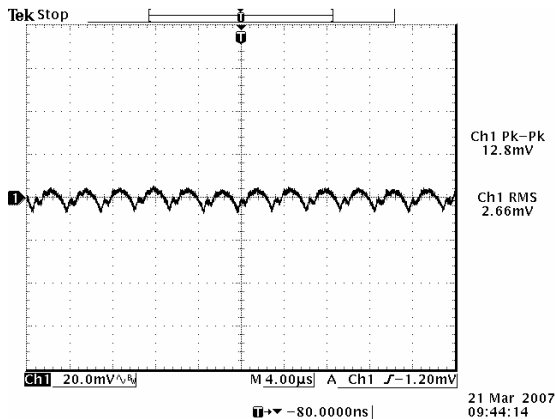
Ripple and noise at no load, 0.8 V output
