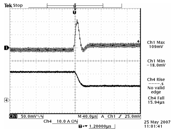
Vout=2.5 V 100% - 50% Load Transients
