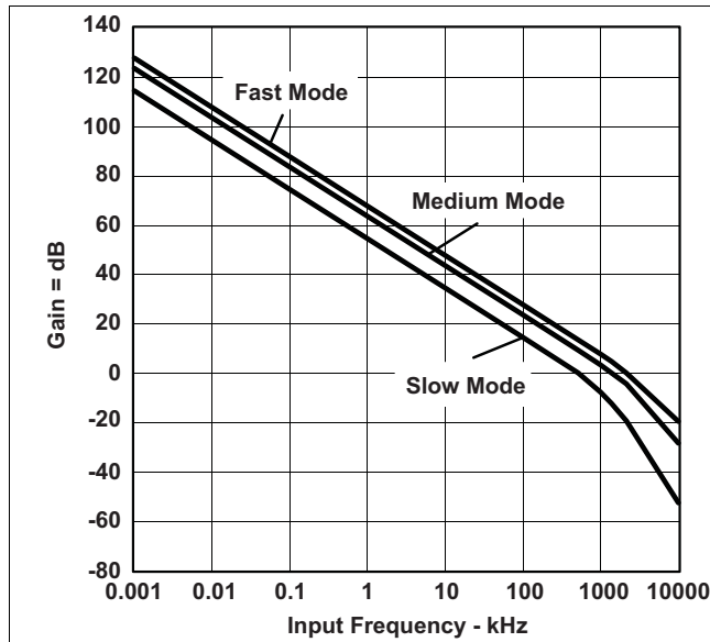
Figure 5-35. Typical Open-Loop Gain vs Frequency
