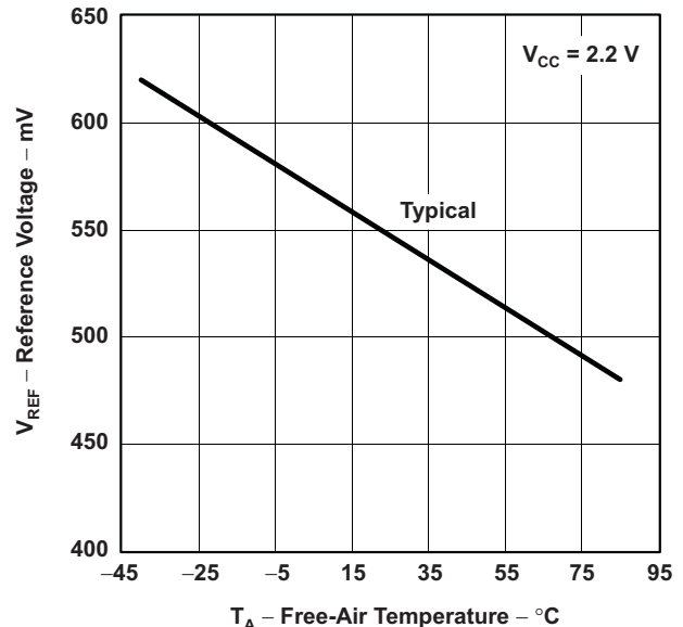
Figure 5-7. Reference Voltage vs Free-Air Temperature
