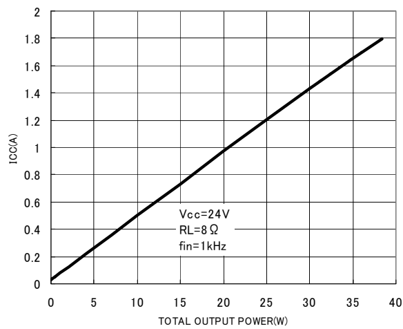
Fig.28 Total output power—Current consumption ( R_L=8\Omega )
