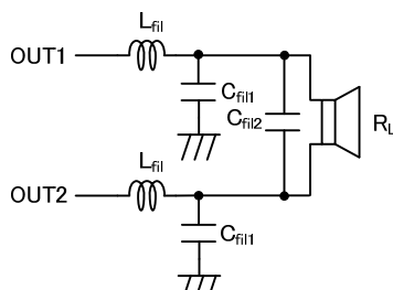
Fig.31 BTL filter configuration
