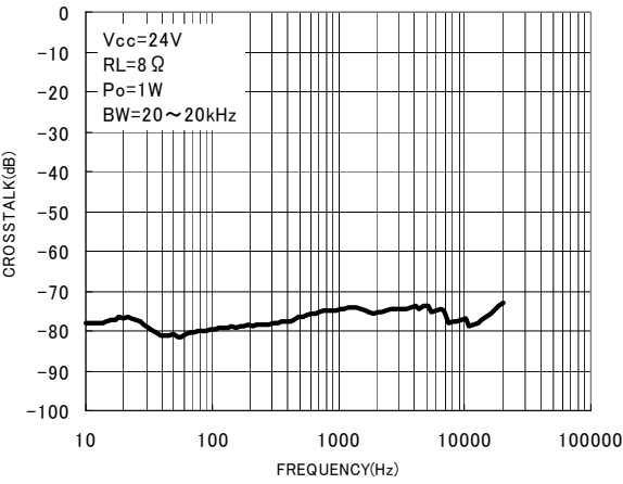
Fig.6 Frequency—Crosstalk
