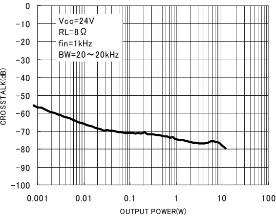
Fig.5 Output power—Crosstalk
