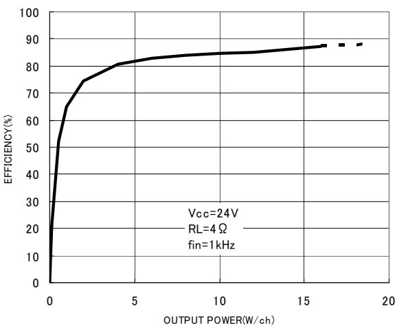
Fig.20 Output power—Efficiency (RL=4Ω)
