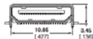
HDMI-C Connector
