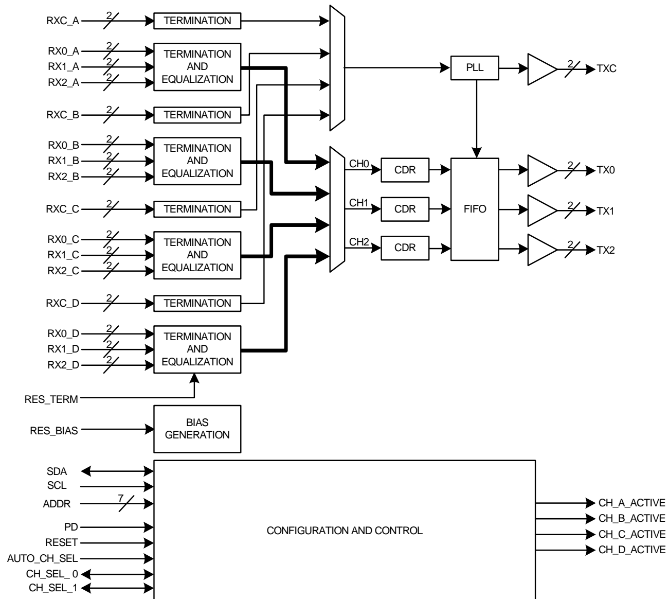
Block Diagram of ISL54100 (ISL54101, ISL54102 identical except for number of channels)
