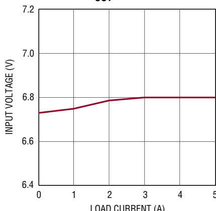
Minimum Required Input Voltage vs Load 5V OUT
