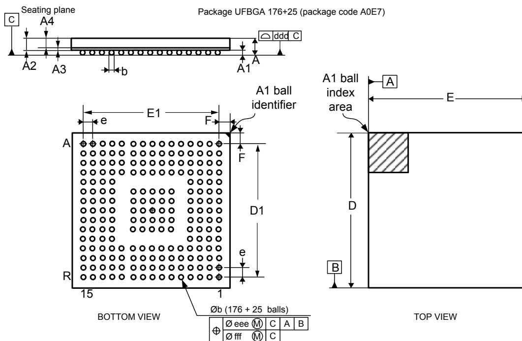
Figure 88. UFBGA(176+25) - Outline
