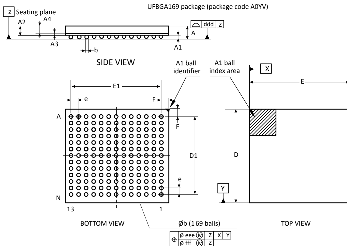
Figure 85. UFBGA169 - Outline
