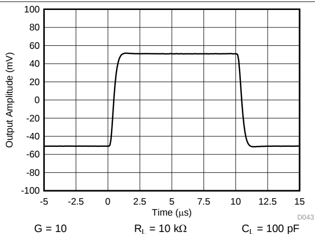
Figure 44. Small-Signal Response
