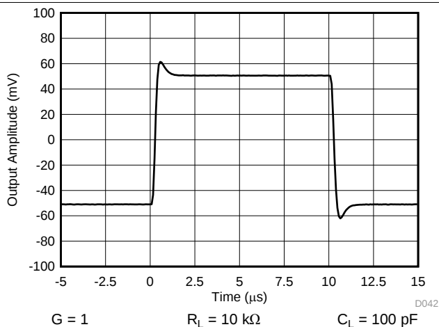
Figure 43. Small-Signal Response
