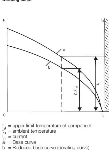
Derating curve
