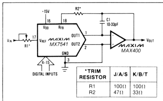
Figure 2. Unipolar Binary Operation
