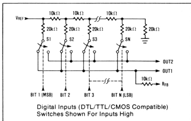
Figure 1. MX7541 Functional Diagram
