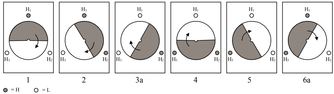
Figure 14. 120° Hall sensor sequence
