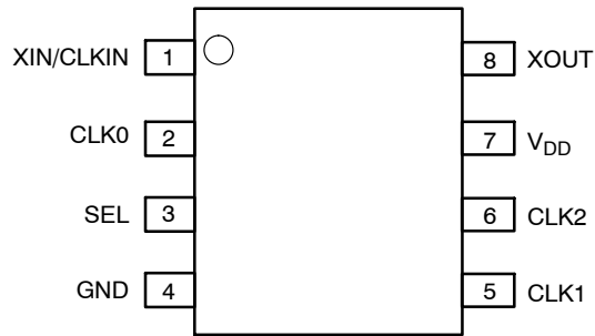
Figure 2. Pin Configuration
